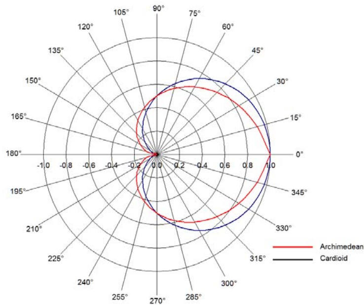
Figure 10. Archimedean spiral and cardioid directivity patterns
