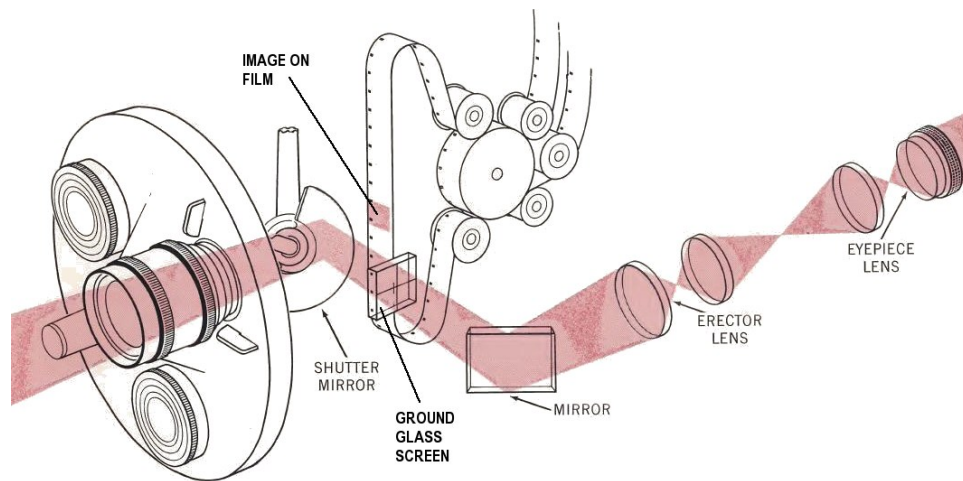
Figure 19. Kodak Reflex Special—reflex viewing system
