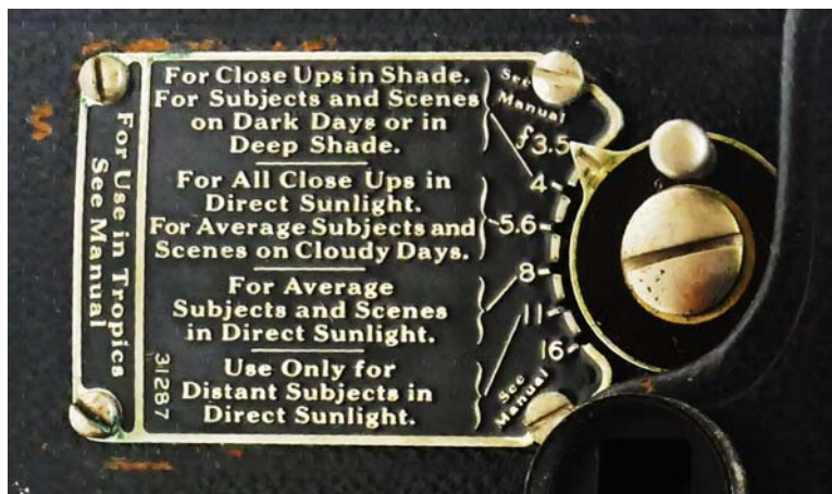
Figure 20. Aperture indicating plate (Ciné-Kodak Model B)
