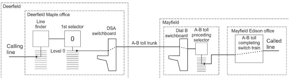
Figure 7. A-B toll call between SXs offices
